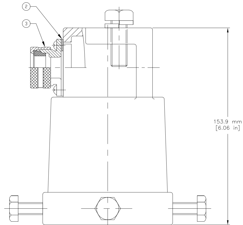
SIDE VIEW
