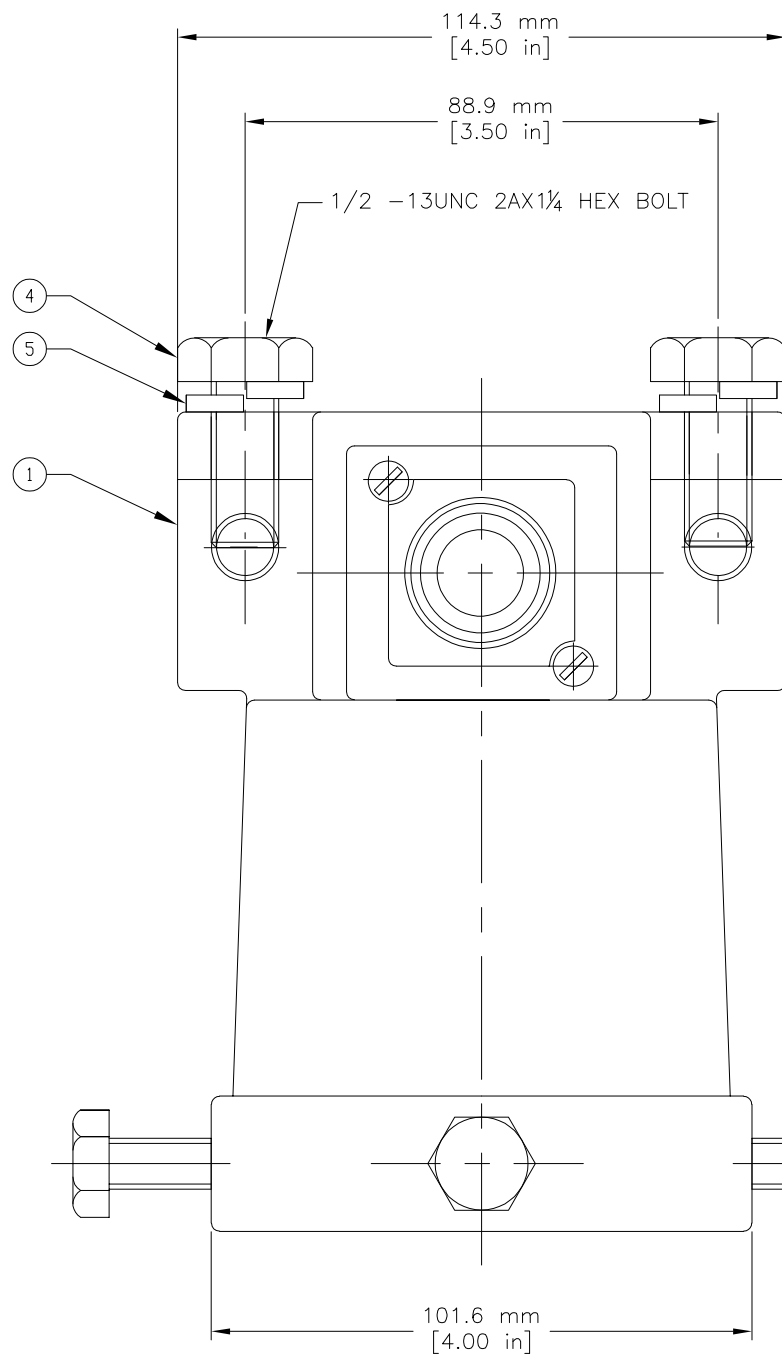
FRONT VIEW
